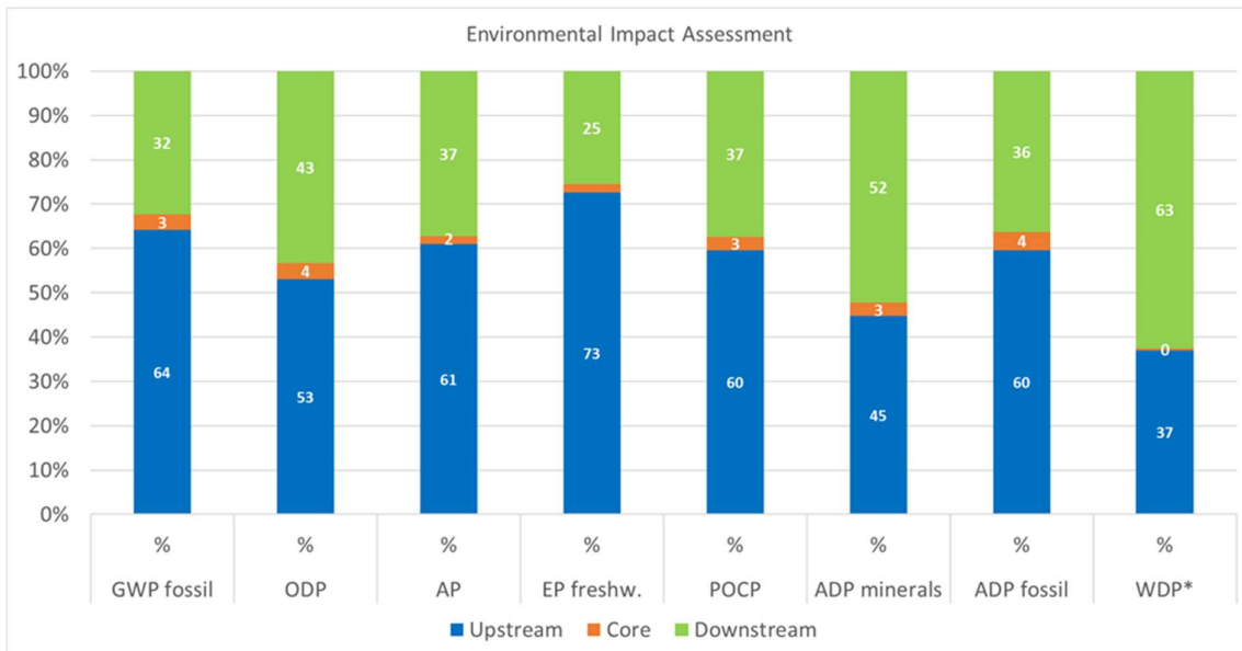
Figure 2. Environmental Impact Assessment of the cable ACSR 25
