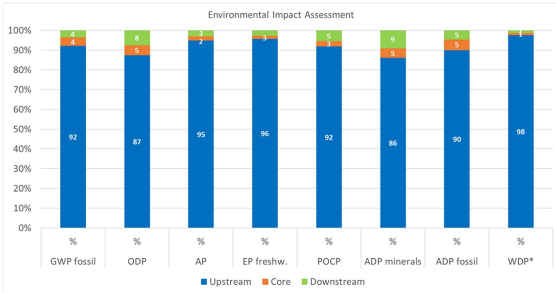
Figure 4. Environmental Impact Assessment of the cable ACSR 281 * Percentage contribution, expressed in absolute value, with respect to the total indicator.
