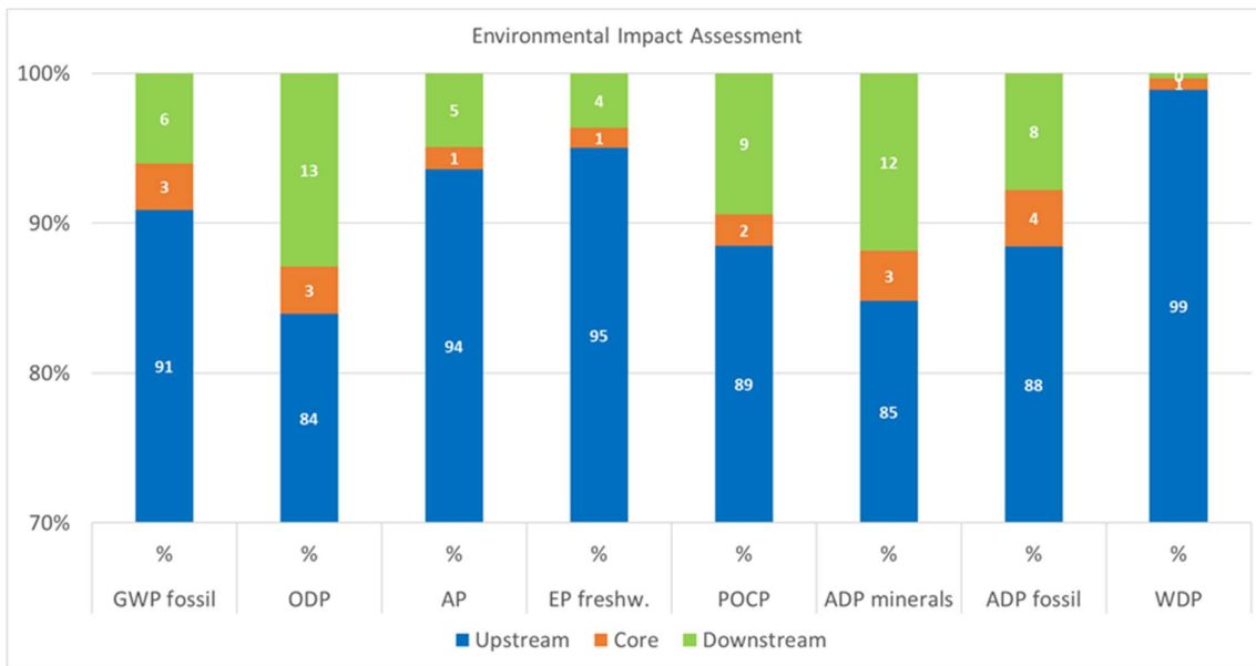
Figure 1. Environmental Impact Assessment of the cable AAAC 500
