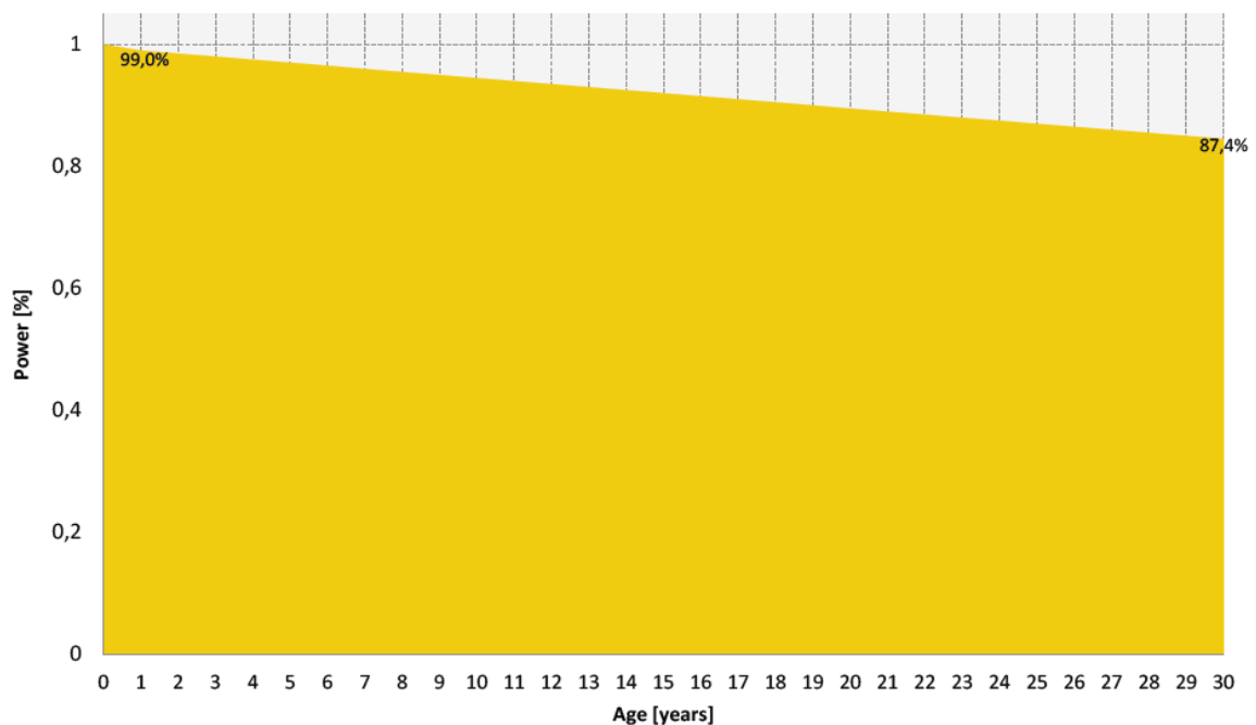
Figure 1: Yearly degradation (30 years)
