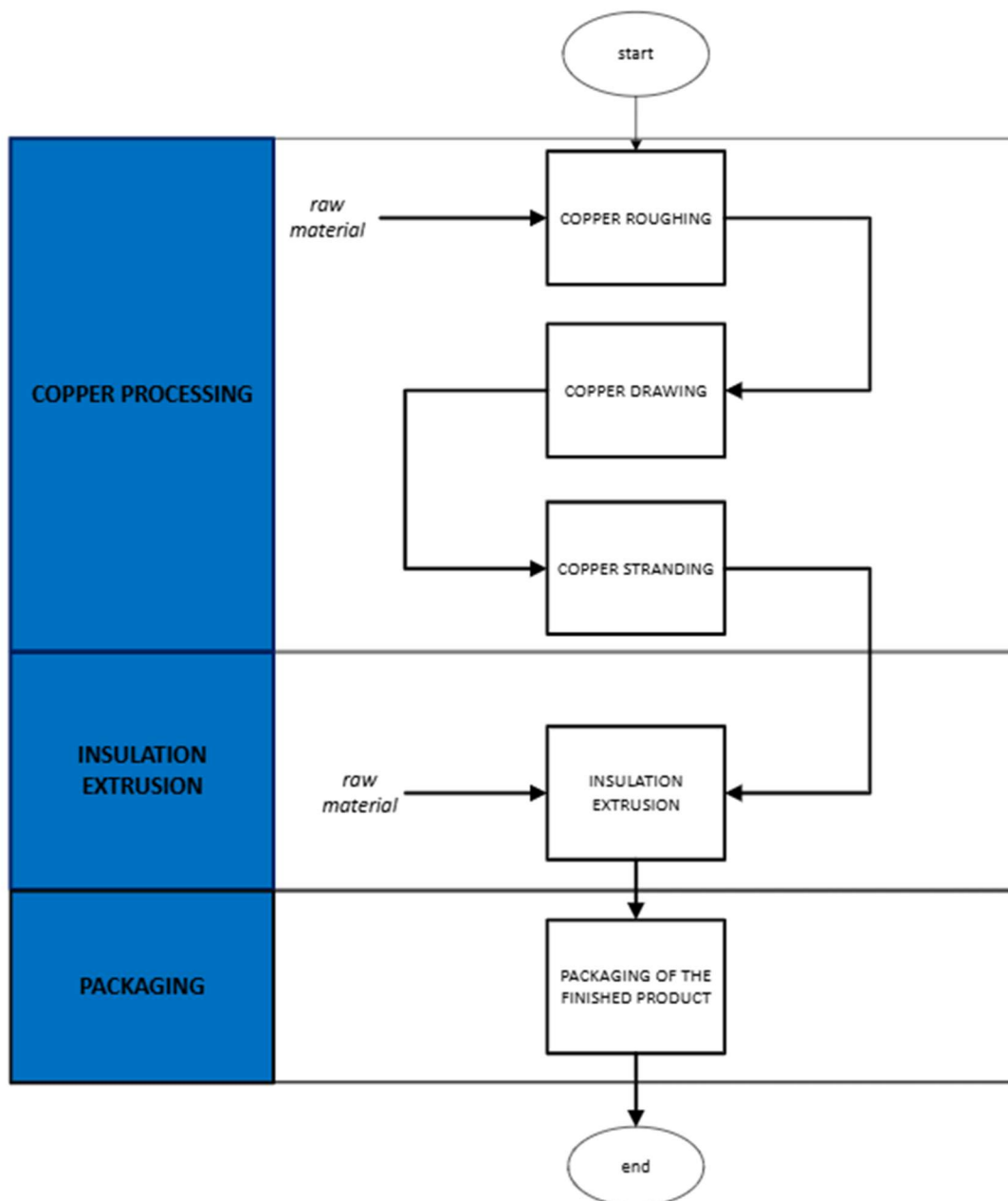
Figure 1. Flowchart
