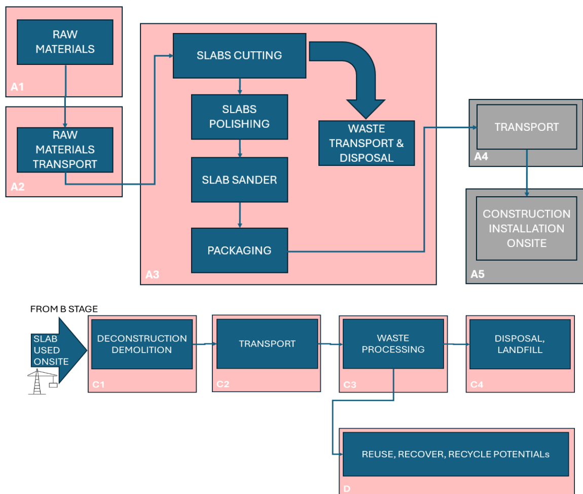
Figure 1: Flow chart of the Eustone Srl production processes and the EPD Life Cycle stages.
