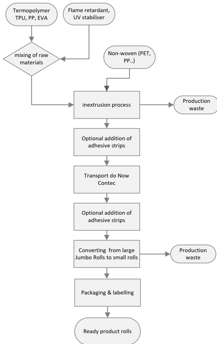
Figure 1 The production flowchart
