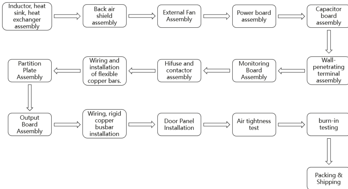
Figure 1 Flow chart of manufacturing energy storage system
