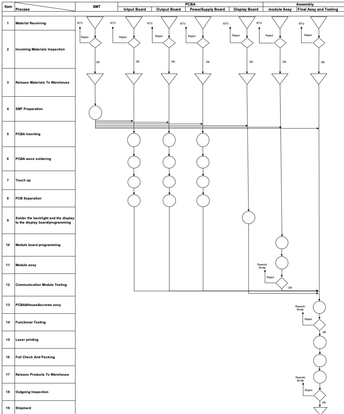
Figure 1. Flow chart of the product EM540DINAV23XM1PFA
