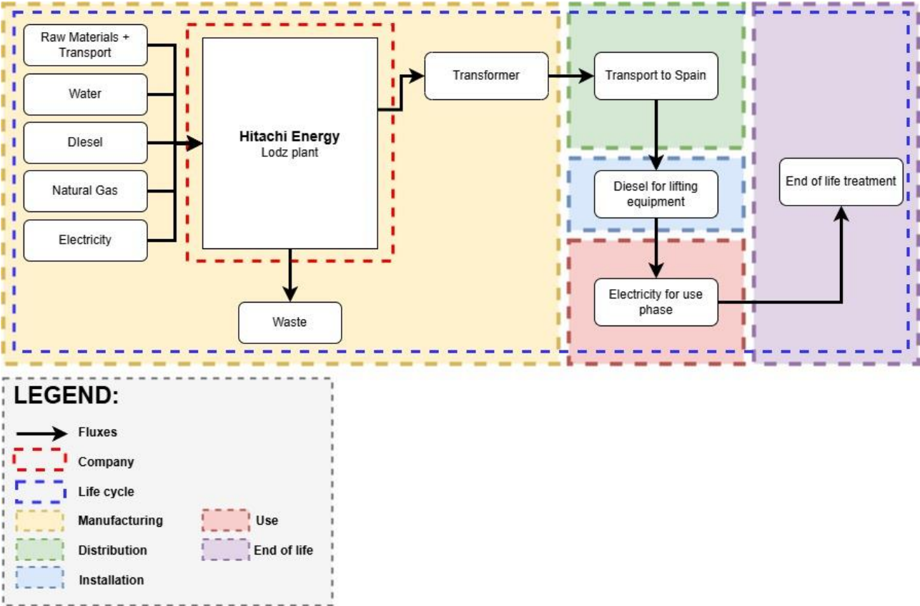
Figure 2 Flux diagram for the product under study
