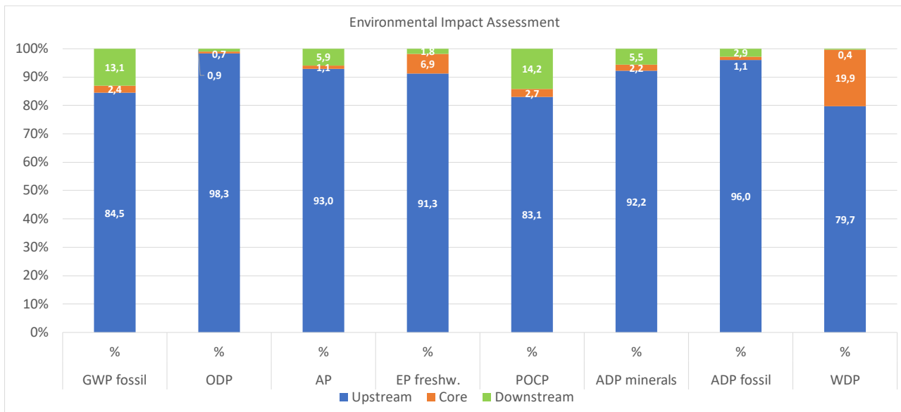
Figure 3. Environmental Impact Assessment of the ARP1H5EX - 3x1x240 cable
