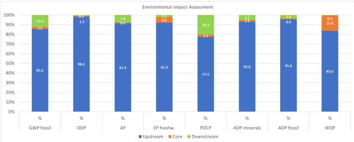
Figure 2. Environmental Impact Assessment of cable ARE4EX 3X1X150+95N
